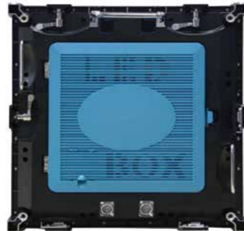
640*640 die-casting cabinet back side
